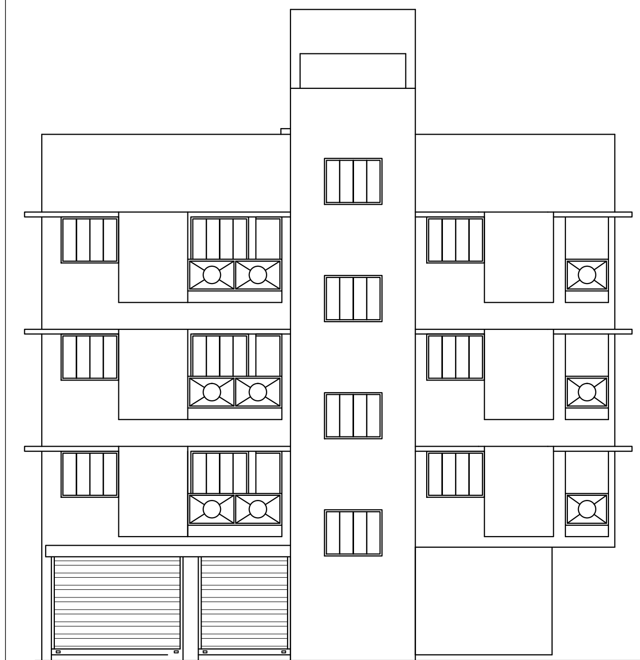
EASTERN SIDE ELEVATION
