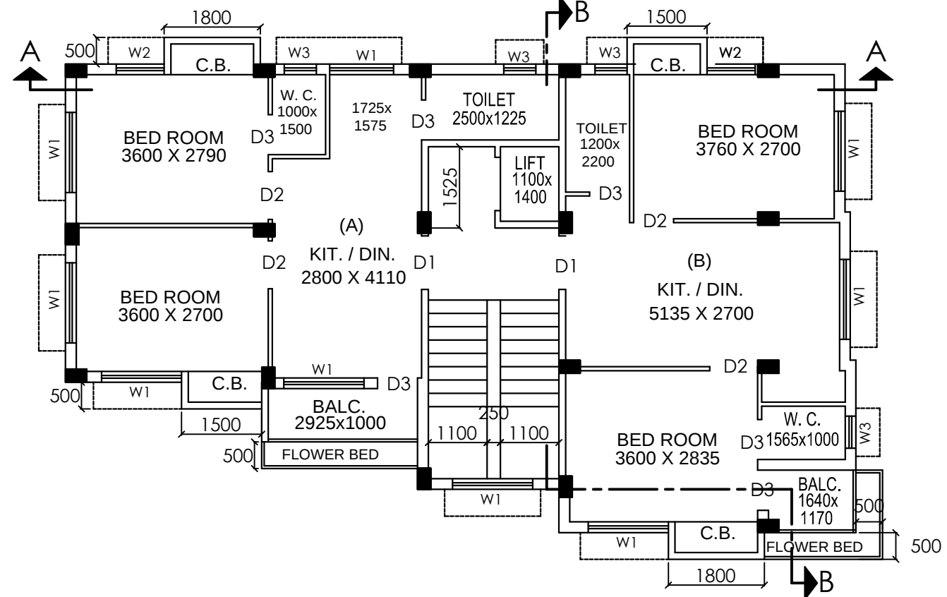
1st, 2nd & 3rd FLOOR PLAN (SCALE-1:100)
